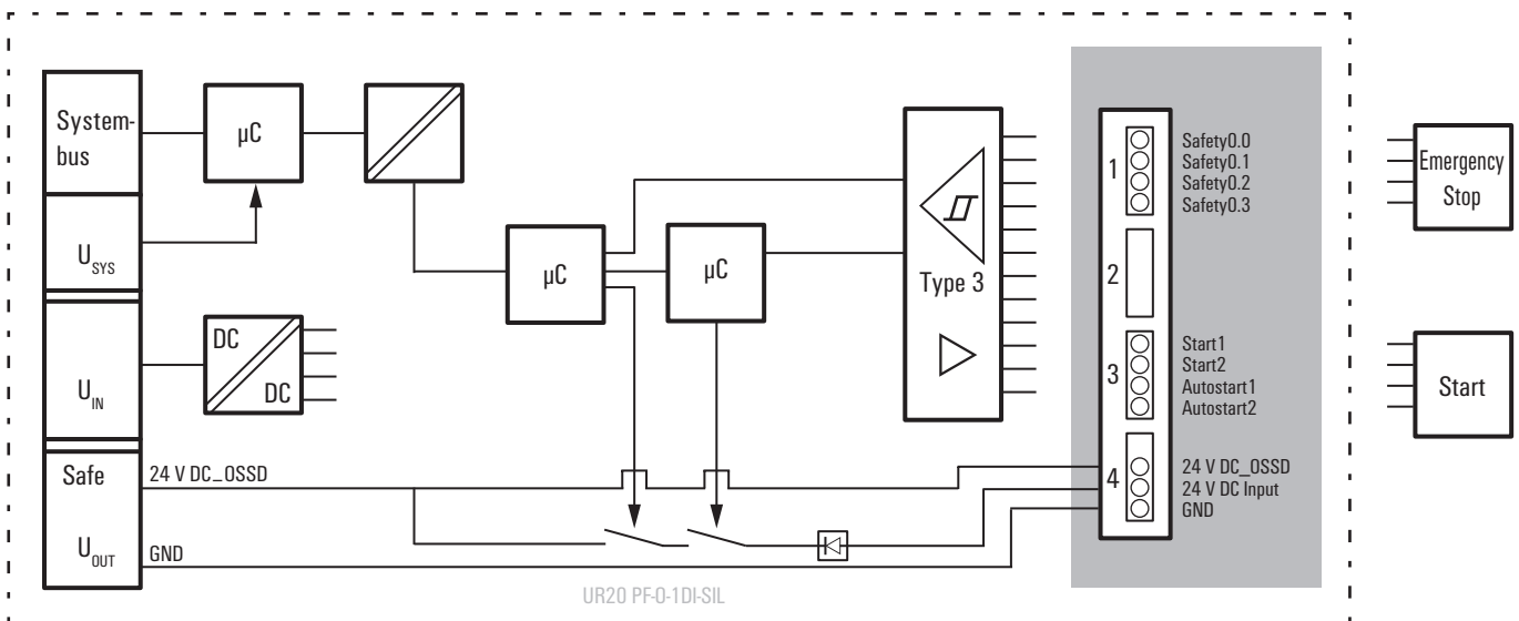
UR20-PF-O-1DI-SIL block diagram example
